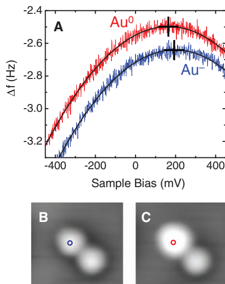
Fig. 3. (A) Frequency shift measured as a function of the voltage above \text{Au}^- and \text{Au}^0 . Both measurements are performed without moving the tip ( A = 0.6 \text{ \AA} and \Delta z = 5.8 \text{ \AA} ; raw data). After measuring \Delta f(V) above \text{Au}^- , the charge state is switched to \text{Au}^0 by applying a bias pulse of V = -1 \text{ V} for a few seconds (26). Parabolic fits and corresponding parabola peaks are indicated. STM images ( I = 7.4 \text{ pA} , V = -50 \text{ mV} , and size = 29 \text{ \AA} by 27 \text{ \AA} ) before (B) and after (C) the \Delta f(V) measurements confirm the charge-switching event and show that the switched Au atom has maintained its lateral position.
