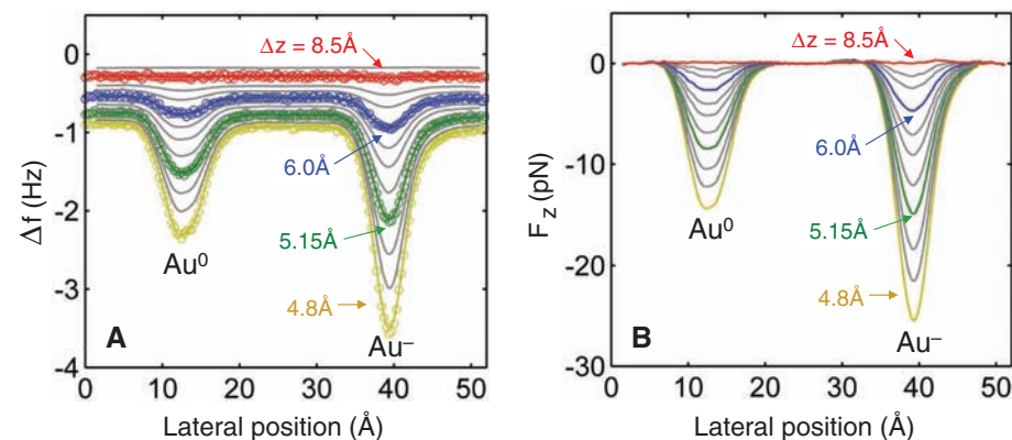
Fig. 2. (A) Frequency shift \Delta f recorded at a constant height ( A = 0.22 Å and V = -2 mV) above \text{Au}^0 and \text{Au}^- . Different line scans correspond to different tip heights \Delta z as indicated. For some curves, every eighth point of the raw data are shown as an open circle in Fig. 2A; the solid lines correspond to the averaged data. (B) Vertical force F_z^* extracted from the averaged data in (A) with the oscillation amplitude deconvolved and the constant background force subtracted from each curve (26).
