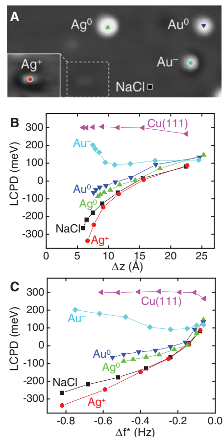
Fig. 4. (A) Constant-current STM image ( I = 3 \text{ pA} , V = 200 \text{ mV} , and size = 130 \text{ \AA} by 60 \text{ \AA} ) of \text{Ag}^+ , \text{Ag}^0 , \text{Au}^0 , and \text{Au}^- on \text{NaCl}(2 \text{ ML})/\text{Cu}(111) . The inset shows the \text{Ag}^+ adatom with fivefold increased z -contrast. (B) LCPD above atoms with different charge states and on \text{NaCl}(2 \text{ ML})/\text{Cu}(111) at the positions indicated in (A) and on \text{Cu}(111) . At each site, \Delta f(V) is measured for different tip heights \Delta z with respect to the NaCl surface [on \text{Cu}(111) with respect to point of contact with the metal]. Each \Delta f(V) measurement is fitted with a parabola, yielding the LCPD and the corresponding frequency shift \Delta f^* . LCPD is shown as a function of \Delta z . (C) LCPD shown as a function of \Delta f^* ; that is, corresponding to a KPFM measurement. The complete set of measurements has been performed without a tip change between measurements (29). Lines serve as a guide to the eye. The errors in \Delta z , LCPD, and \Delta f^* estimated from repeated measurements are \pm 0.2 \text{ \AA} , \pm 15 \text{ meV} , and \pm 30 \text{ mHz} , respectively.
