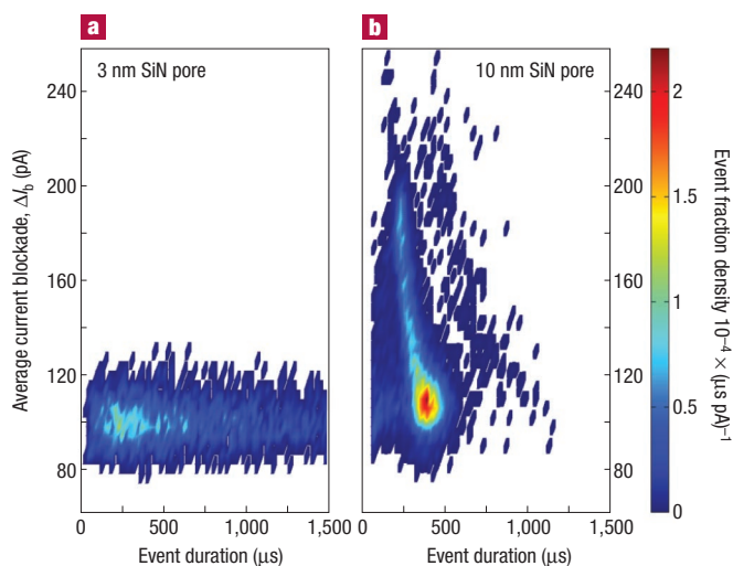
Figure 2 Distribution of events as a function of t_d and \langle\Delta I_b\rangle for 10-kb dsDNA. a , A 3-nm pore, 2,674 events; b , a 10-nm pore, 9,477 events. The bias voltage was 120 mV. The colour scale represents event-fraction density normalized as a probability distribution so that the integral of the density over all t_d and \langle\Delta I_b\rangle is equal to 1.
